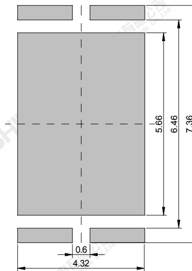
recommended stencil pattern
